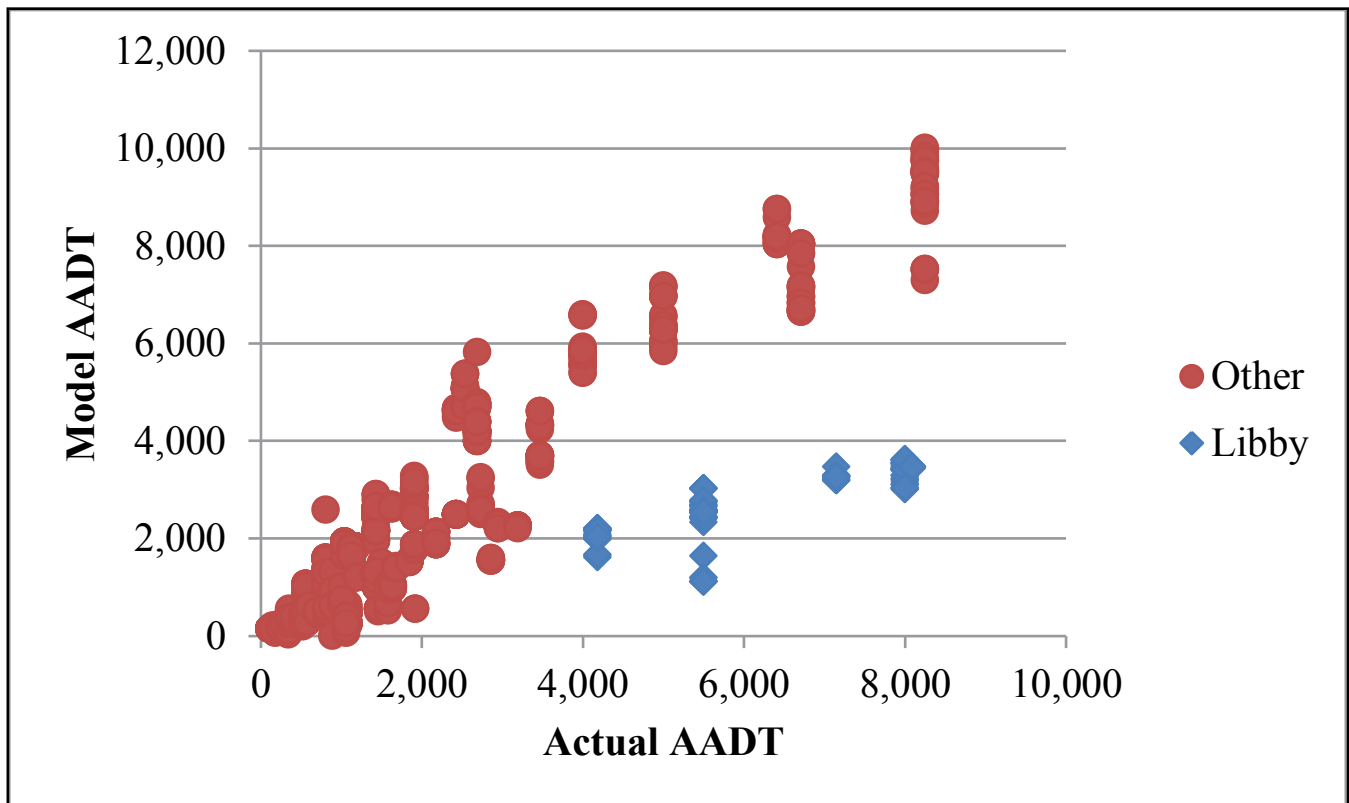
Figure 25: A comparison of current modeled traffic with actual traffic in the study area validated the model.
